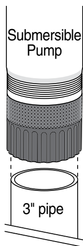
Figure 1: Insert a 3" PVC pipe in the bottom of the motor to raise the pump in the tank.
